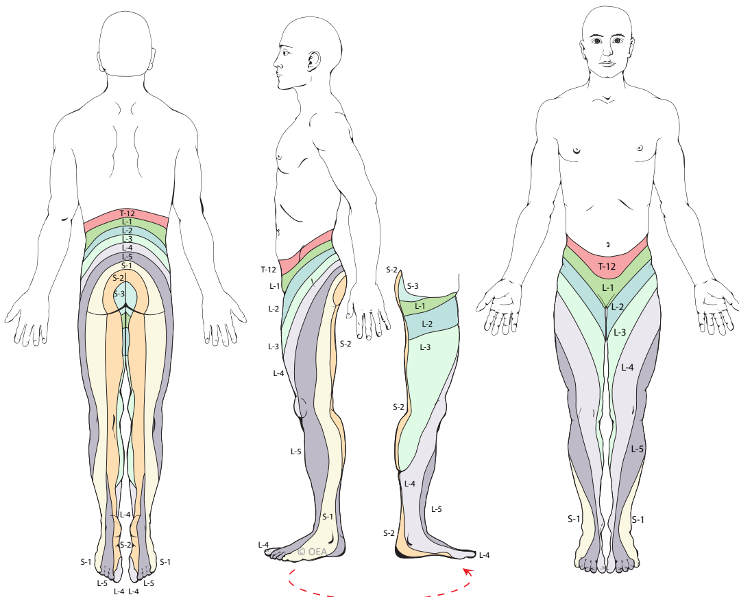
Lumbar Dermatomes
